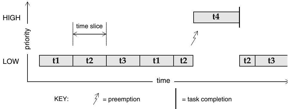
Figure 3-3 Round-Robin Scheduling
