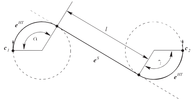
Figure 2: The shortest path example between two configurations c_1 and c_2 .
