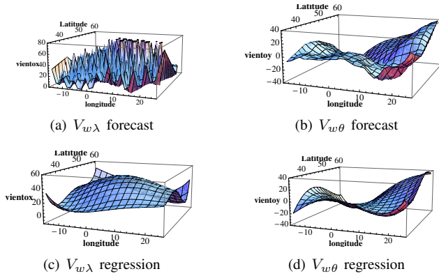
Fig. 1. Wind data at 250 [Hpa] -h=10395 [m]-
