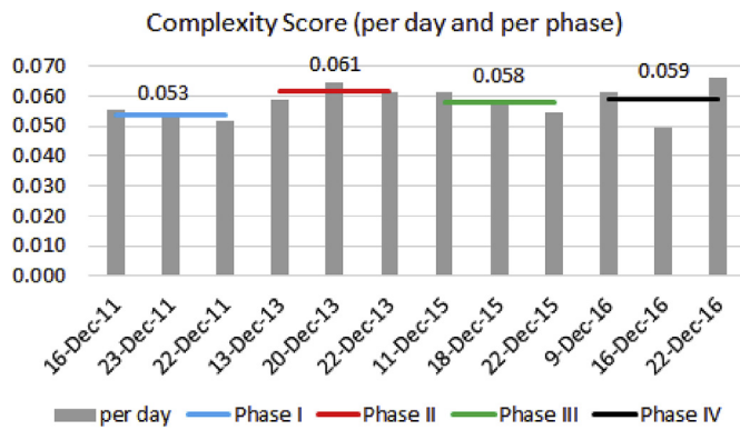
Fig. 6. Complexity score.
