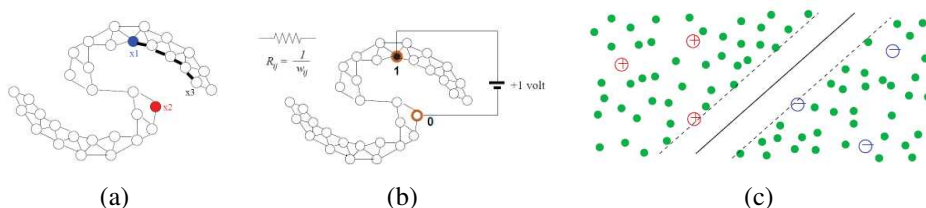
Figure 5.22 Examples of semi-supervised learning ( Zhu and Goldberg 2009 ) © 2009 Morgan & Claypool: (a) two labeled samples and a graph connecting all of the samples; (b) solving binary labeling with harmonic functions, interpreted as a resistive electrical network; (c) using semi-supervised support vector machine (S3VM).
