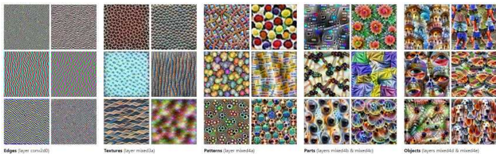
Figure 5.49 Feature visualization of how GoogLeNet (Szegedy, Liu et al. 2015) trained on ImageNet builds up its representations over different layers, from Olah, Mordvintsev, and Schubert (2017).
