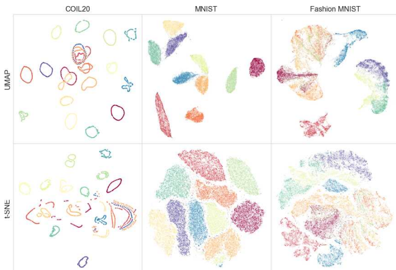
Figure 5.21 Comparison of UMAP and t-SNE manifold learning algorithms © McInnes, Healy, and Melville (2018) on three different computer vision learning recognition tasks: COIL ( Nene, Nayar, and Murase 1996 ), MNIST ( LeCun, Cortes, and Burges 1998 ), and Fashion MNIST ( Xiao, Rasul, and Vollgraf 2017 ).
