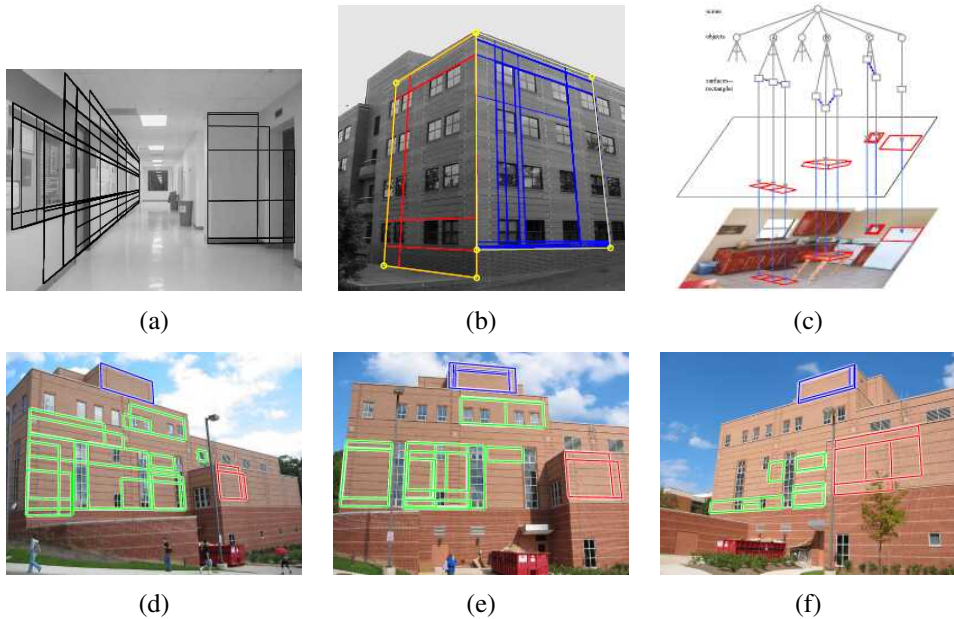
Figure 7.51 Rectangle detection: (a) indoor corridor and (b) building exterior with grouped facades (Kořecká and Zhang 2005) © 2005 Elsevier; (c) grammar-based recognition (Han and Zhu 2005) © 2005 IEEE; (d–f) rectangle matching using a plane sweep algorithm (Mičušík, Wildenauer, and Kořecká 2008) © 2008 IEEE.
