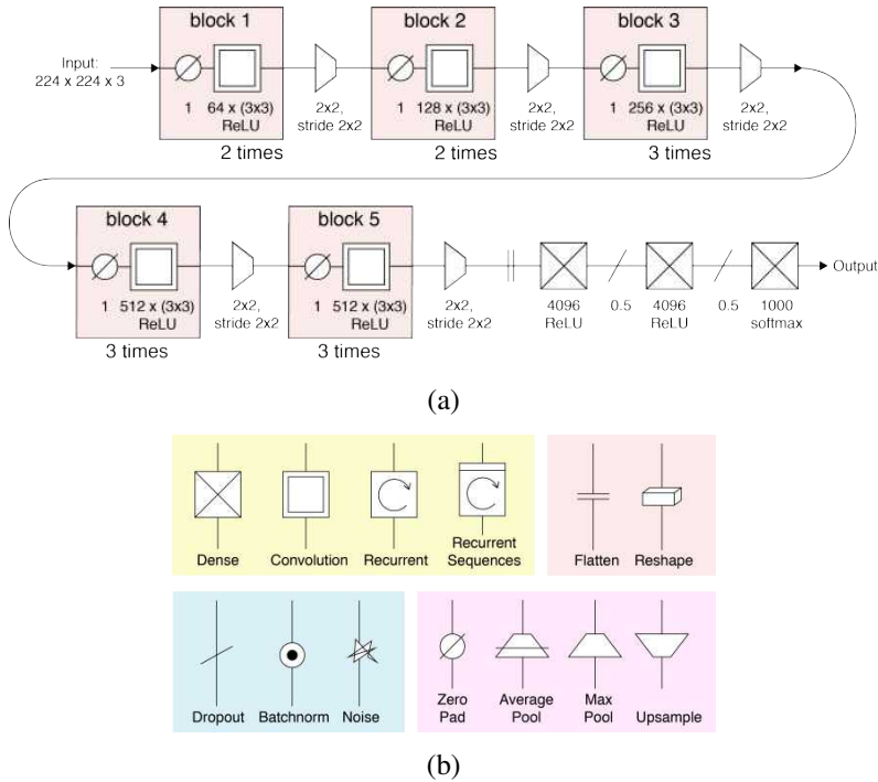
Figure 5.41 The VGG16 network of Simonyan and Zisserman (2014b) © Glassner (2018) . (a) The network consists of repeated zero-pad, 3 \times 3 convolution, ReLU blocks interspersed with 2 \times 2 max pooling and a doubling in the number of channels. This is followed by some fully connected and dropout layers, with a final softmax into the 1,000 ImageNet categories. (b) Some of the schematic neural network symbols used by Glassner (2018) .
