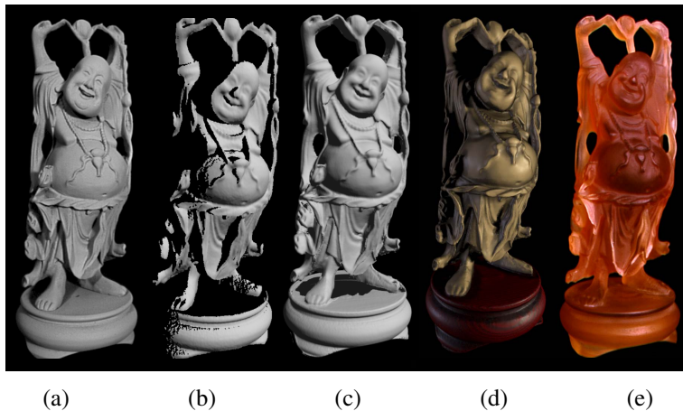
Figure 13.12 Reconstruction and hardcopy of the “Happy Buddha” statuette ( Curless and Levoy 1996 ) © 1996 ACM: (a) photograph of the original statue after spray painting with matte gray; (b) partial range scan; (c) merged range scans; (d) colored rendering of the reconstructed model; (e) hardcopy of the model constructed using stereolithography.
