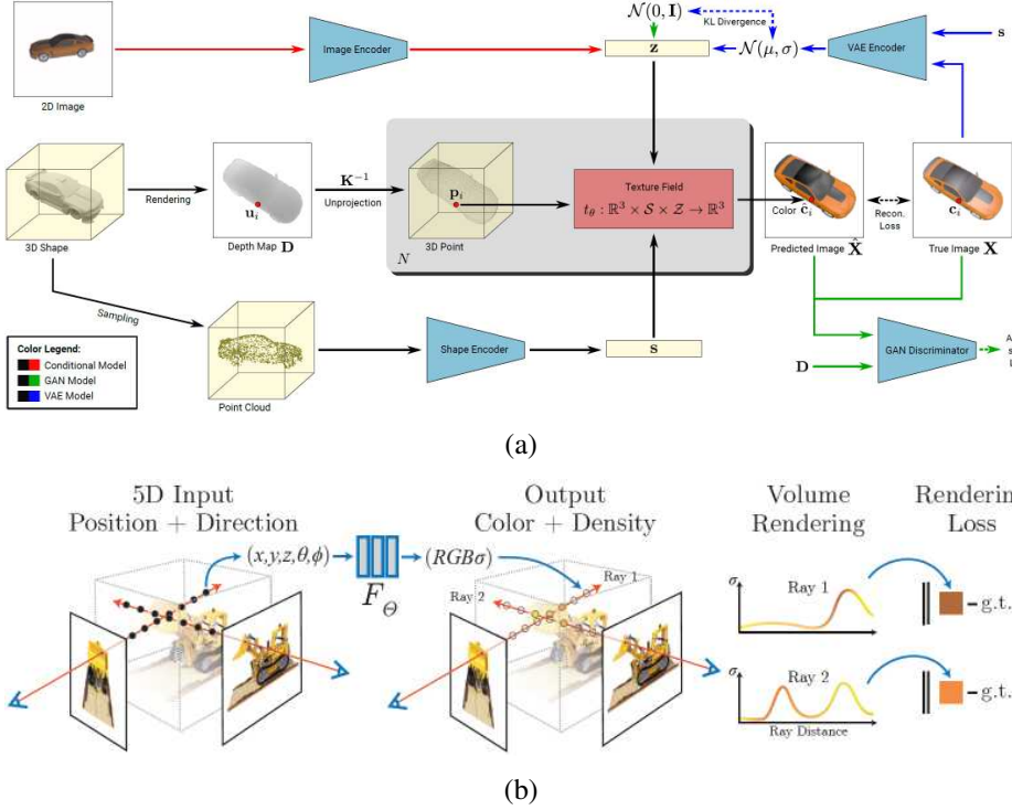
Figure 14.24 Examples of implicit function (MLP) neural rendering: (a) Texture Fields (Oechsle, Mescheder et al. 2019) © 2019 IEEE; (b) Neural Radiance Fields (Mildenhall, Srinivasan et al. 2020) © 2020 Springer.
