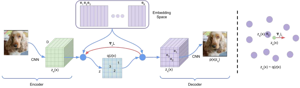
Figure 5.58 The VQ-VAE model. On the left, z_e(x) represents the output of the encoder, the embedding space on top represents the codebook of K embedding vectors, and q(z|x) represents the process of replacing each spatial (i.e., channel-wise) vector in the output of the encoder with its nearest vector in the codebook. On the right, we see how a z_e(x) vector (green) may be rounded to e_2 , and that the gradient in the encoder network (red) may push the vector away from e_2 during backpropagation. © van den Oord, Vinyals, and Kavukcuoglu (2017)
