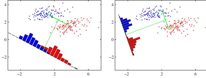
Figure 5.10 Fisher linear discriminant (Bishop 2006) © 2006 Springer. To find the projection direction to best separate two classes, we compute the sum of the two class covariances and then use its inverse to rotate the vector between the two class means.
