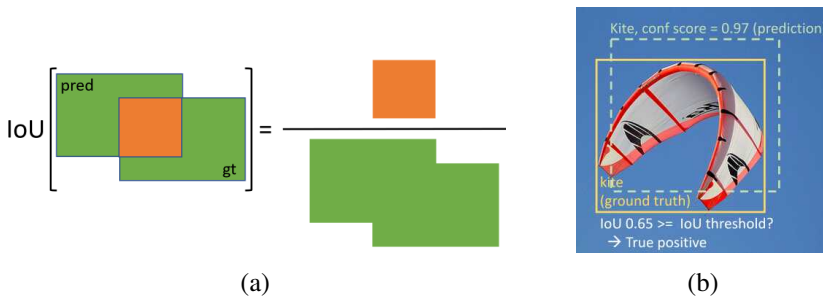
Figure 6.26 Intersection over union (IoU): (a) schematic formula, (b) real-world example © 2020 Ross Girshick.
