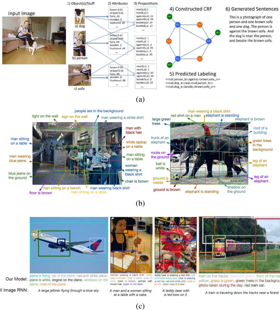
Figure 6.45 Image captioning systems: (a) BabyTalk detects objects, attributes, and positional relationships and composes these into image captions (Kulkarni, Premraj et al. 2013) © 2013 IEEE; (b–c) DenseCap associates word phrases with regions and then uses an RNN to construct plausible sentences (Johnson, Karpathy, and Fei-Fei 2016) © 2016 IEEE.
