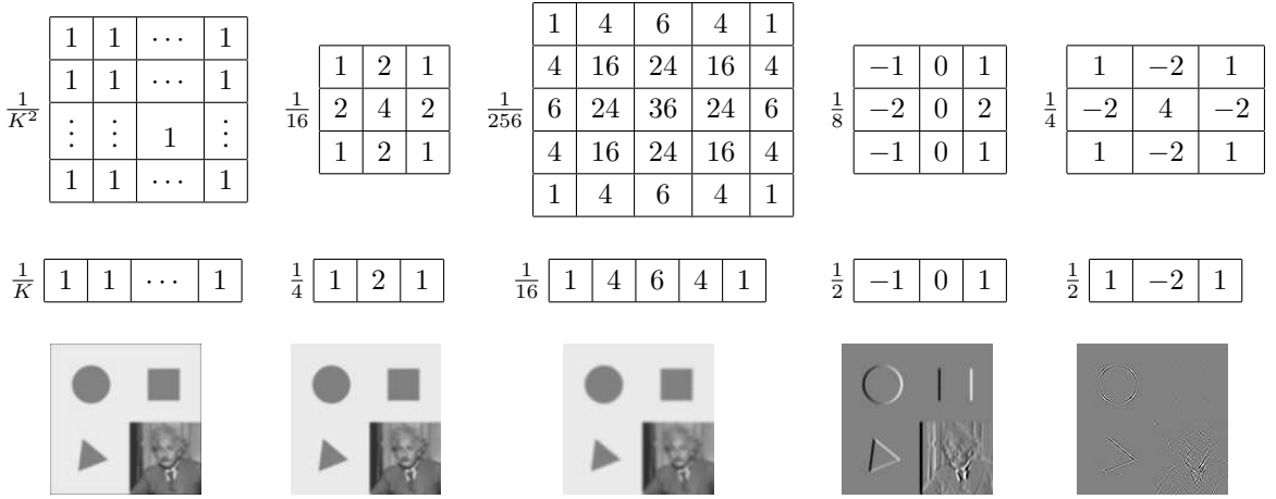
(a) box, K = 5 (b) bilinear (c) "Gaussian" (d) Sobel (e) corner
