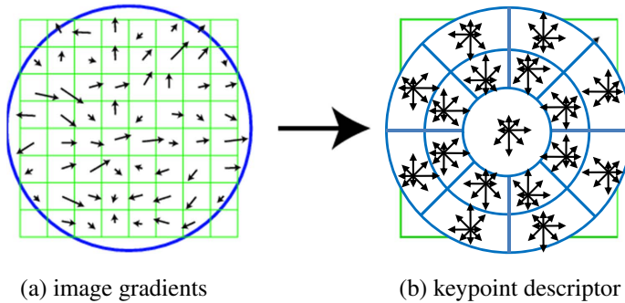
Figure 7.17 The gradient location-orientation histogram (GLOH) descriptor uses log-polar bins instead of square bins to compute orientation histograms (Mikolajczyk and Schmid 2005). GLOH uses 16 gradient orientations inside each bin, although this figure only shows 8 to appear less cluttered.
