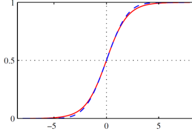
Figure 5.7 The logistic sigmoid function \sigma(l) , shown in red, along with a scaled error function, shown in dashed blue (Bishop 2006) © 2006 Springer.
