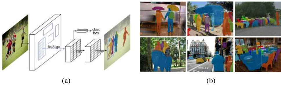
Figure 6.36 Instance segmentation using Mask R-CNN (He, Gkioxari et al. 2017) © 2017 IEEE: (a) system architecture, with an additional segmentation branch; (b) sample results.
